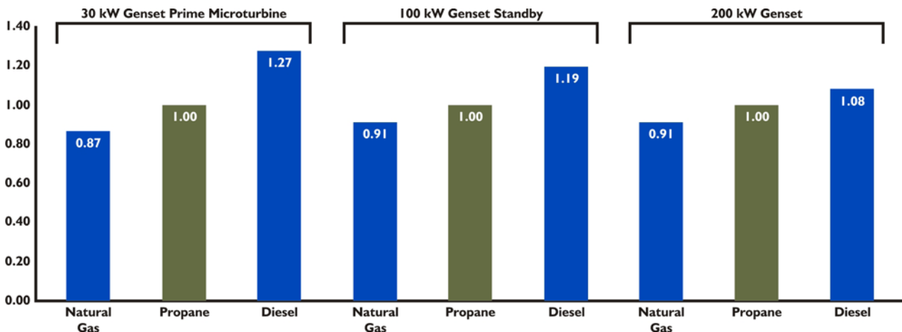
Figure 4.9. Distributed Generation
